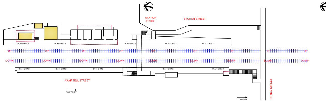
FOOTBRIDGE LEVEL
